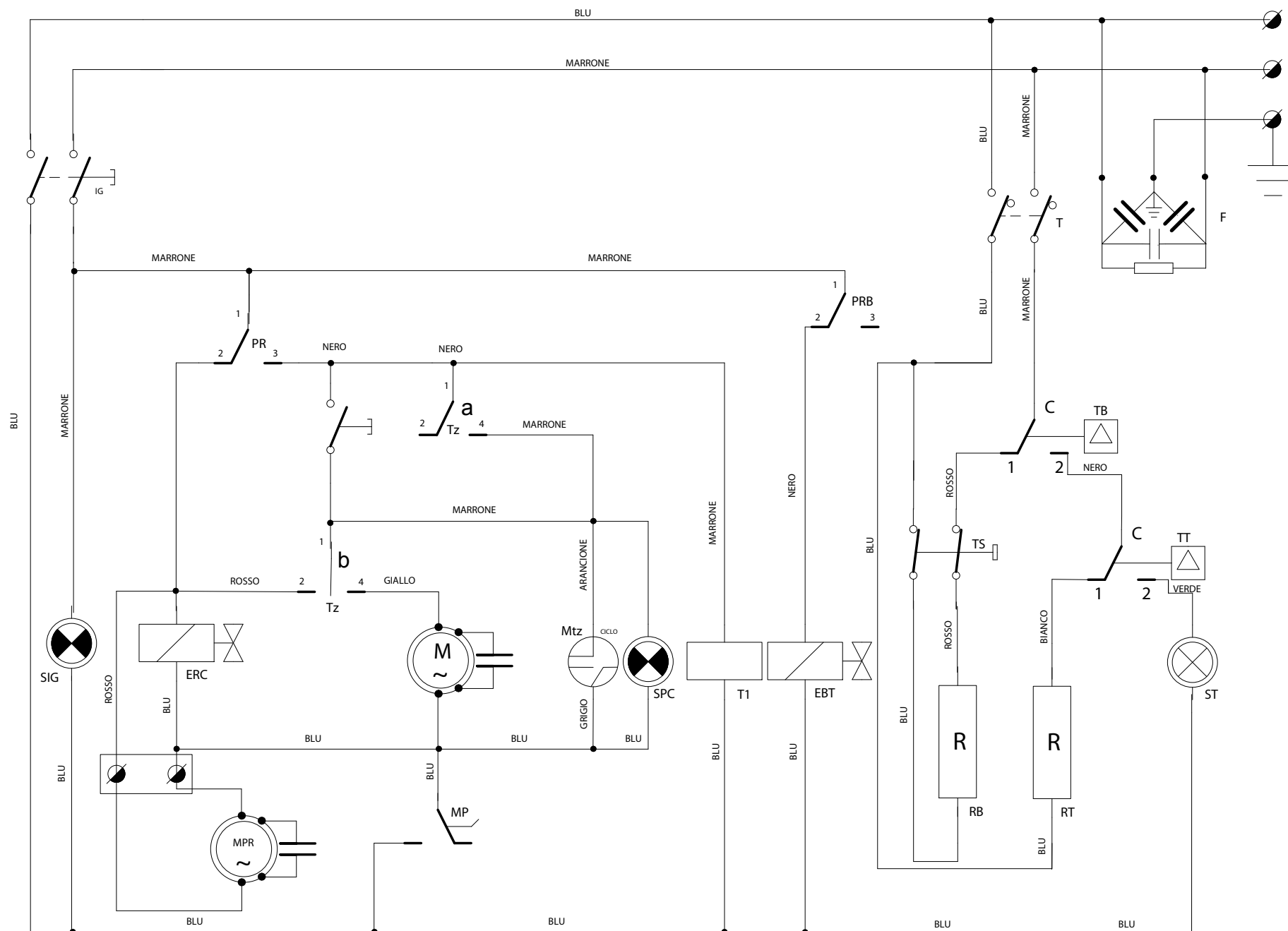
Midi50-Breaktank 230V~50Hz
